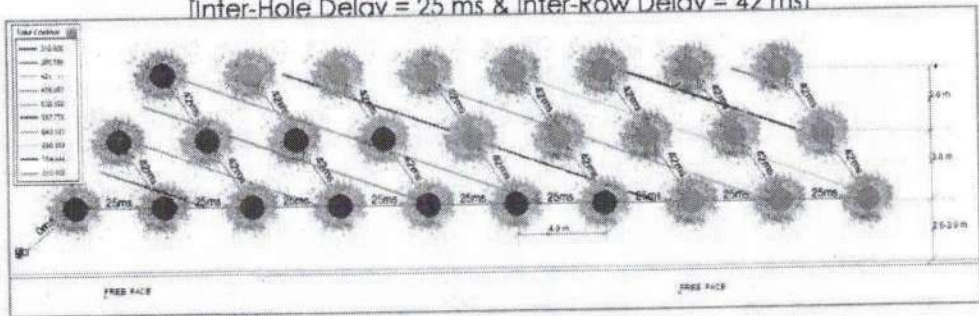
Fig. 7.10: Diagonal sequence of rock movement and time contour obtained from the recommended firing patterns in Figures 7.9
