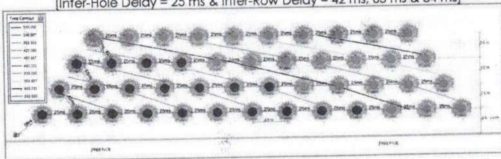
Fig. 7.12: Diagonal sequence of rock movement and time contour obtained from the recommended firing patterns in Figures 7.11
