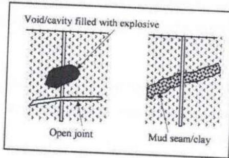
(E) Cavity, open joint and mud seam
