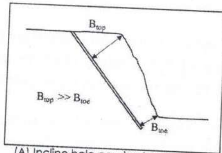
(A) Incline hole causing less toe burden
