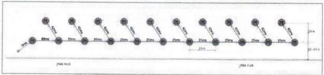
Fig. 7.5. Another recommended drilling and surface hole-to-hole firing pattern for controlled blasting operations within 100 - 200 m from the Railway Line [Inter-Hole Delay = 25 ms & Inter-Row Delay = 42 ms]
