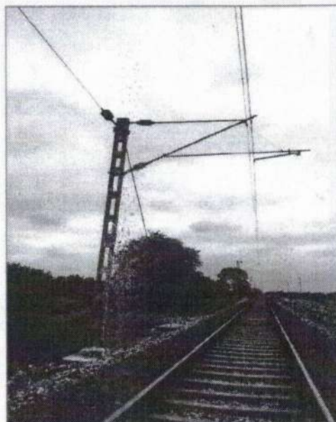
Plate 5.3. View of the Overhead Line Electrifications
