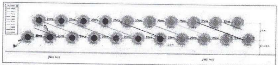
Fig. 7.4: Diagonal sequence of rock movement and time contour obtained from the recommended firing pattern in Figures 7.3
