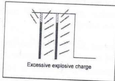
(F) Excessive charge and very small top stemming
