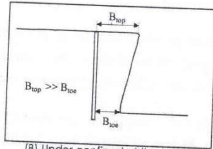
(B) Under-confined at the toe
