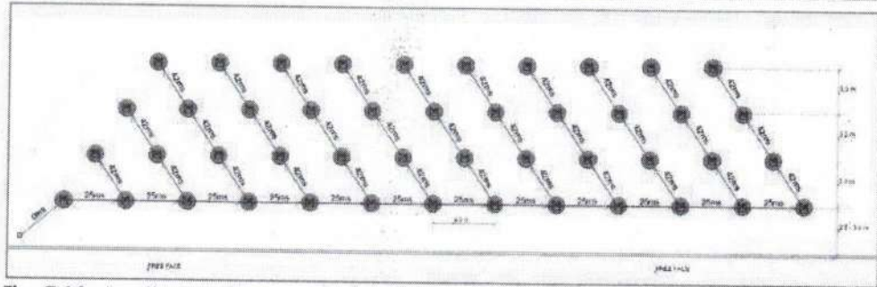
Fig. 7.13. Another recommended drilling and surface hole-to-hole firing pattern for controlled blasting operations beyond 300 m of the Railway Line [Inter-Hole Delay = 25 ms & Inter-Row Delay = 42 ms]
