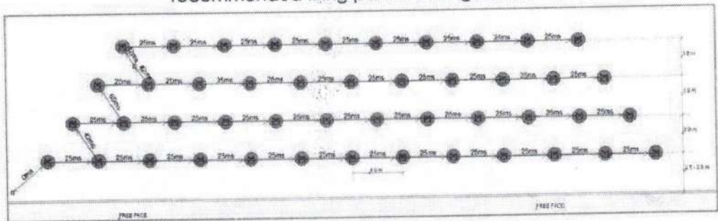
Fig. 7.11. Recommended drilling and surface hole-to-hole firing pattern for controlled blasting operations beyond 300 m of the Railway Line [Inter-Hole Delay = 25 ms & Inter-Row Delay = 42 ms, 65 ms & 84 ms]
