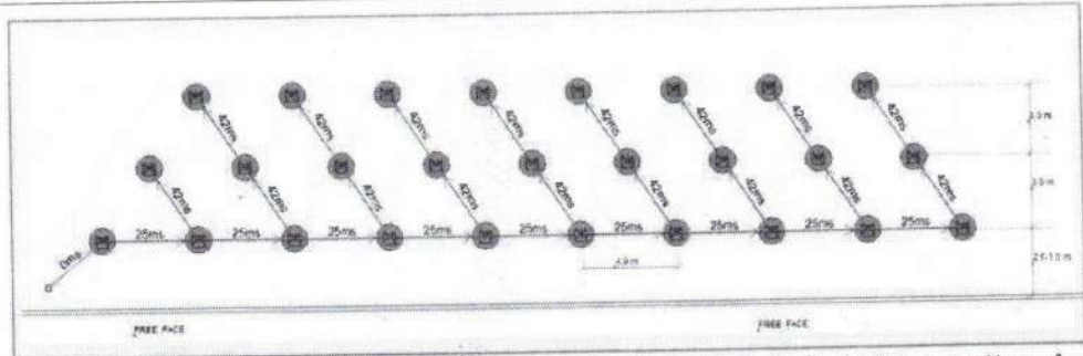
Fig. 7.9. Another recommended drilling and surface hole-to-hole firing pattern for controlled blasting operations within 200 - 300 m from the Railway Line [Inter-Hole Delay = 25 ms & Inter-Row Delay = 42 ms]
