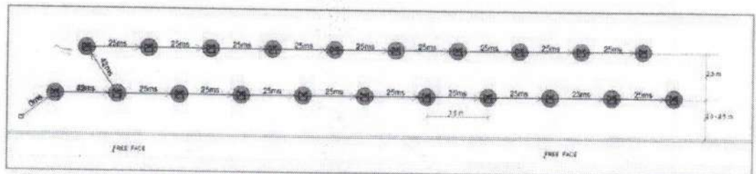
Fig. 7.3. Recommended drilling and surface hole-to-hole firing pattern for controlled blasting operations within 100 - 200 m from the Railway Line [Inter-Hole Delay = 25 ms & Inter-Row Delay = 42 ms]
