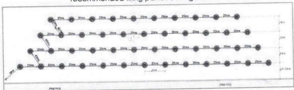
Fig. 7.11. Recommended drilling and surface hole-to-hole firing pattern for controlled blasting operations beyond 300 m of the Railway Line [Inter-Hole Delay = 25 ms & Inter-Row Delay = 42 ms, 65 ms & 84 ms]
